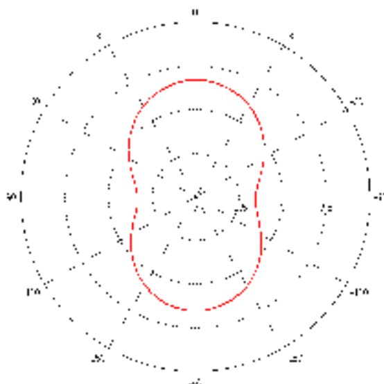
Plano H
